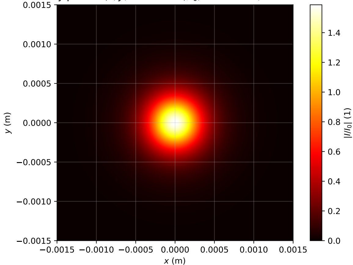
Intensity profile I(x, y, z = 1.592m)/I_0 , Pin=0.9Pcr, artificial time
